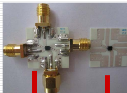
3dB 90 ° Hybrid Coupler
