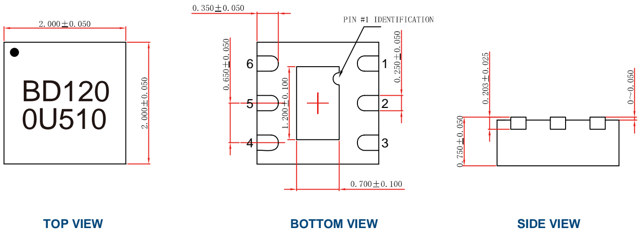
TOP VIEW
