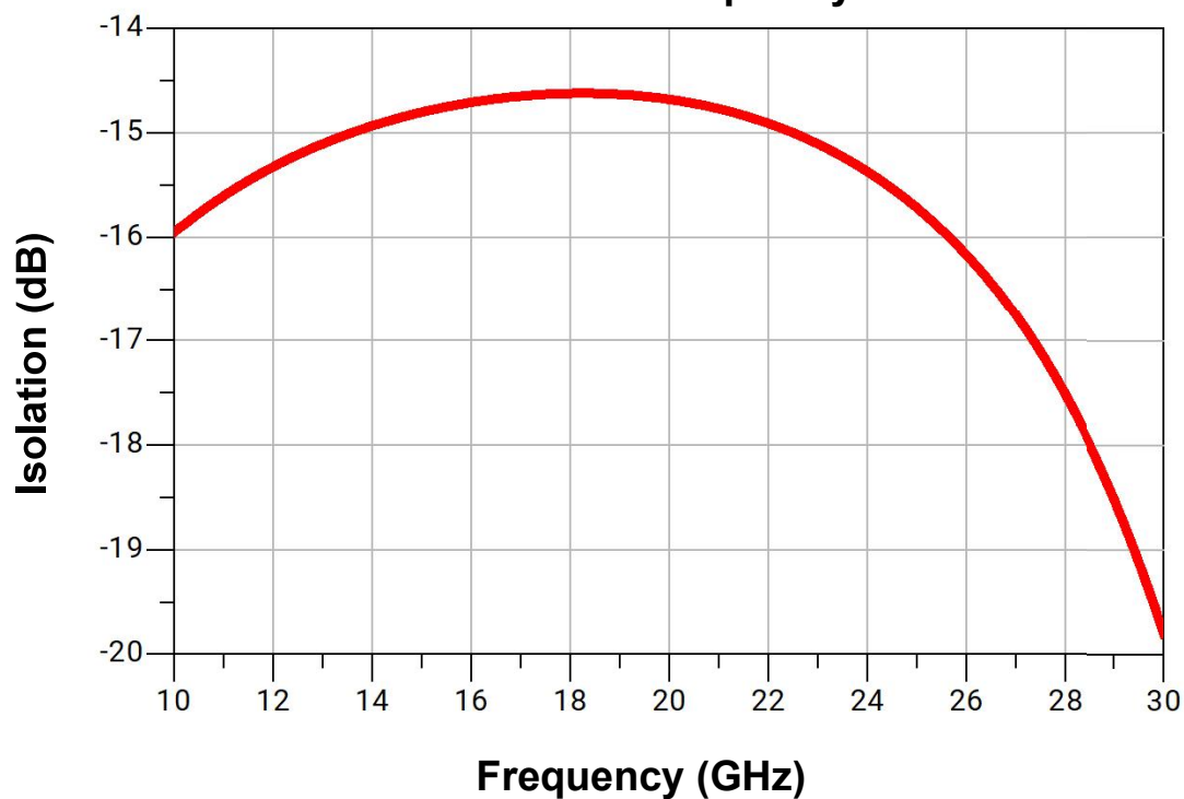
Isolation VS.Frequency
