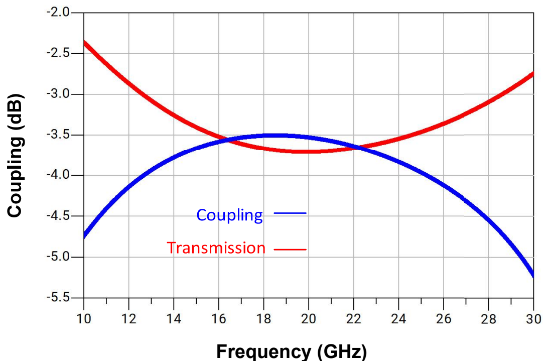
Insertion Loss VS.Frequency
