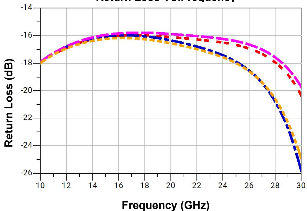
Return Loss VS.Frequency
