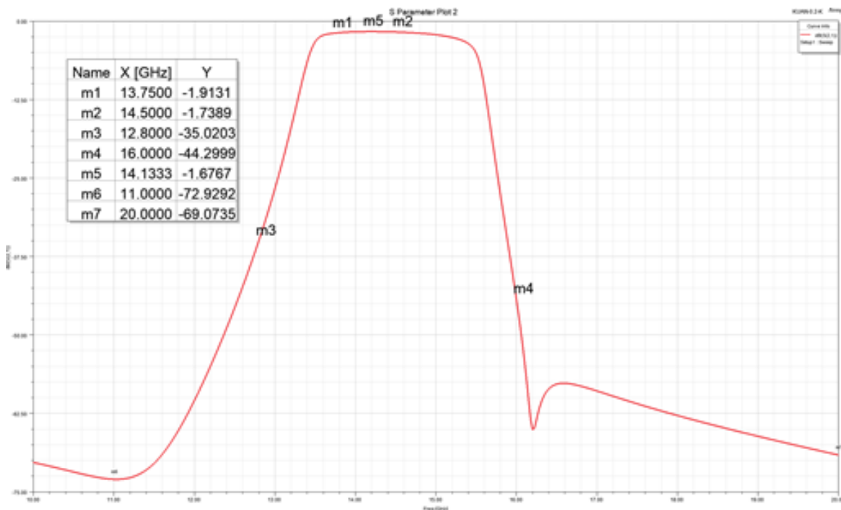
插入损耗-S21
